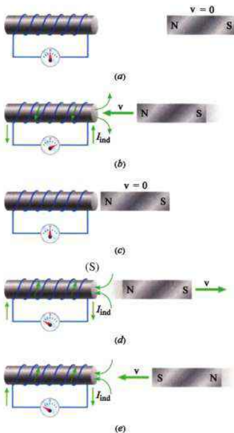
Fig ( 3 - 2 ) Lenz's law
