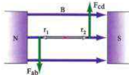
b) top view (plan) of the rectangle when the coil is parallel to the field.
