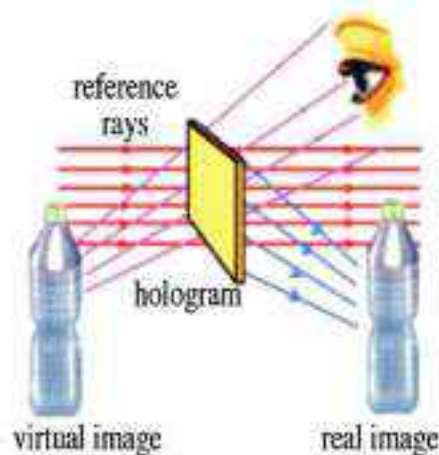
Fig ( 7-12b) Hologram as a grating
