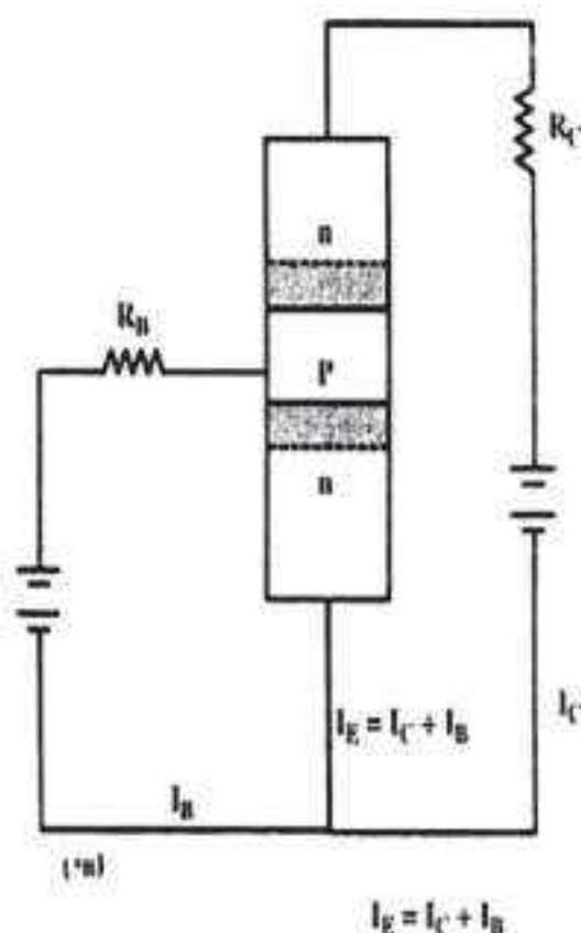
Fig ( 8-17b) A transistor amplifier with a common emitter
