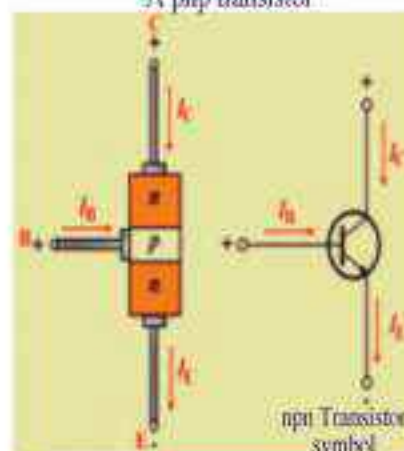
Fig (8-16d) An npn transistor
