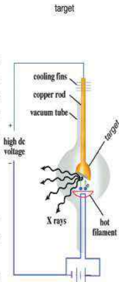
Fig (6- 6 ) Coolidge tube
