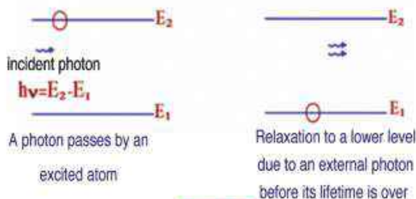
Fig ( 7 -2) Stimulated emission
