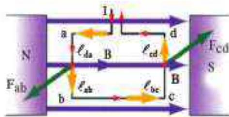
a) the coil is parallel to the magnetic field.
