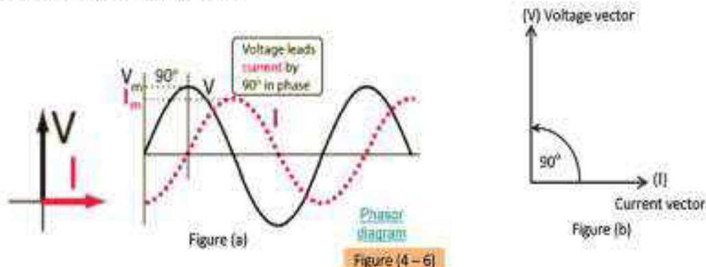
Figure (4 - 6) AC voltage leads AC current in an inductor by 90^\circ
